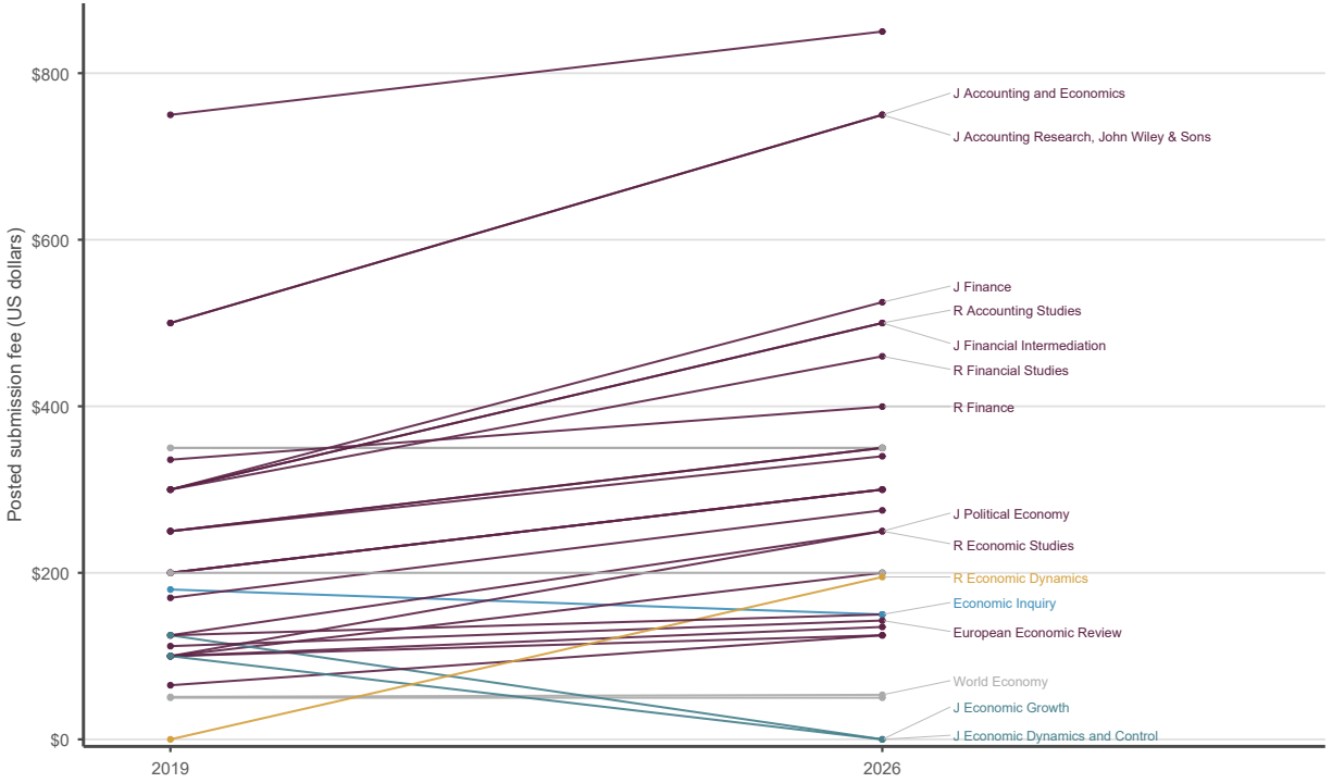
Figure 2: Posted submission fees in 2019 and 2026. Each line is one of the 32 matched journals whose endpoints are directly comparable: both positive in the same posted currency, introduced from zero or removed to zero. Plum lines raised the fee, blue lines lowered it, grey lines left it unchanged, the gold line introduced a fee and teal lines removed one. Classes are assigned within the posted currency. For display, euro and sterling amounts are converted to dollars at European Central Bank reference rates: the 2019 annual averages of 1.12 and 1.28, and the census-month averages of 1.14 and 1.34 for July 2026. Twenty-eight further journals were at zero in both years and five required membership in 2019. One more changed its posted currency and cannot be compared. None of those groups is drawn. The unit of observation is a matched journal.
