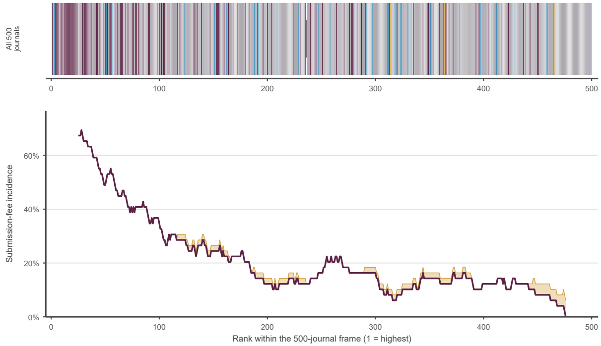
Figure 1: The census of submission fees, July 2026. The upper panel draws one tick per journal in the frame, in rank order, coloured by evidence class: plum ticks charge for submission, blue ticks carry text stating that no submission charge applies, light grey ticks show no charge after the prescribed search, gold ticks are unresolved and the short dark tick admits only members. The lower panel plots the share charging (plum line) within a centred 49-journal window of the 500-journal frame. The gold band raises every unresolved record in the window to a charger. The unit of observation is a journal. The band measures classification sensitivity, not sampling uncertainty.
