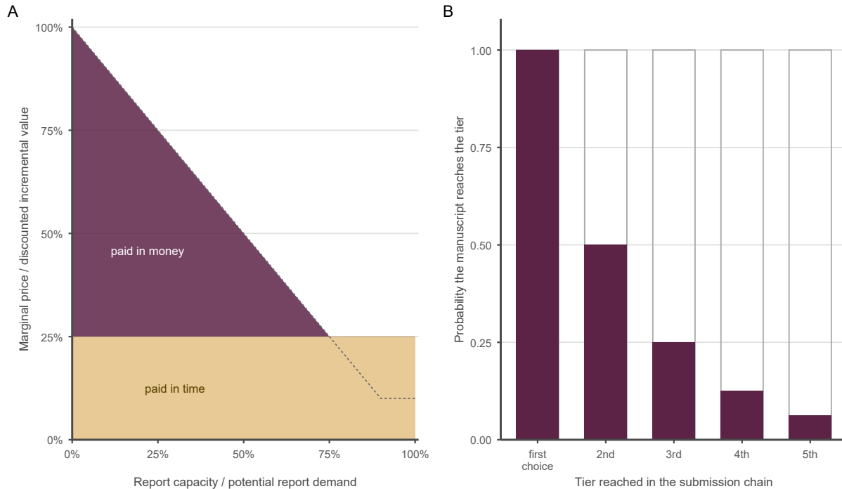
Figure 3: Money, delay and routing in the benchmark model. Panel A shows the price that clears report capacity under uniform beliefs, as a share of the discounted incremental value of placement. The marginal entrant always bears the delay burden (gold), set at 25 per cent of that value. The money fee (plum) is the residual above the delay floor and reaches zero while capacity is still scarce. The dashed line repeats the schedule for a 10 per cent burden. The horizontal axis is report capacity divided by the report demand that every potential manuscript would generate. Panel B shows the probability that one manuscript reaches each of five tiers when half of rejected authors continue after each rejection (solid bars), against complete continuation (outlined bars). Expected attempts per manuscript, equation (6), are 1.94 and five. Both panels are theoretical scenario maps. No line is fitted to posted fees.
