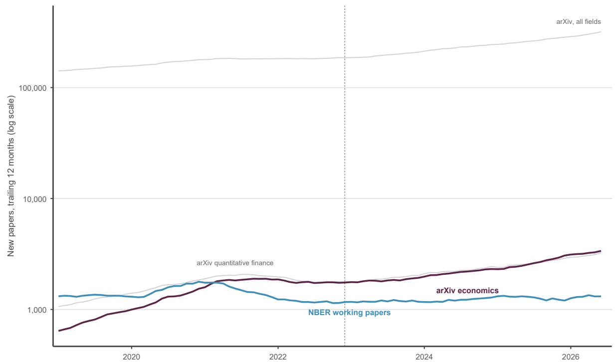
Figure 4: Manuscript growth where posting is open and where it is gated. Twelve-month trailing totals of new papers, log scale. The dashed line marks the release of ChatGPT. In the year to June 2026 arXiv economics grew 0.28 log points while the affiliation-gated NBER series was approximately flat. The grey series show arXiv in all fields and in quantitative finance for scale. The unit is a posted paper rather than a journal submission or a report request.
